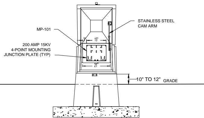
1 PHASE FRONT ELEVATION VIEW (DOOR OPEN)
