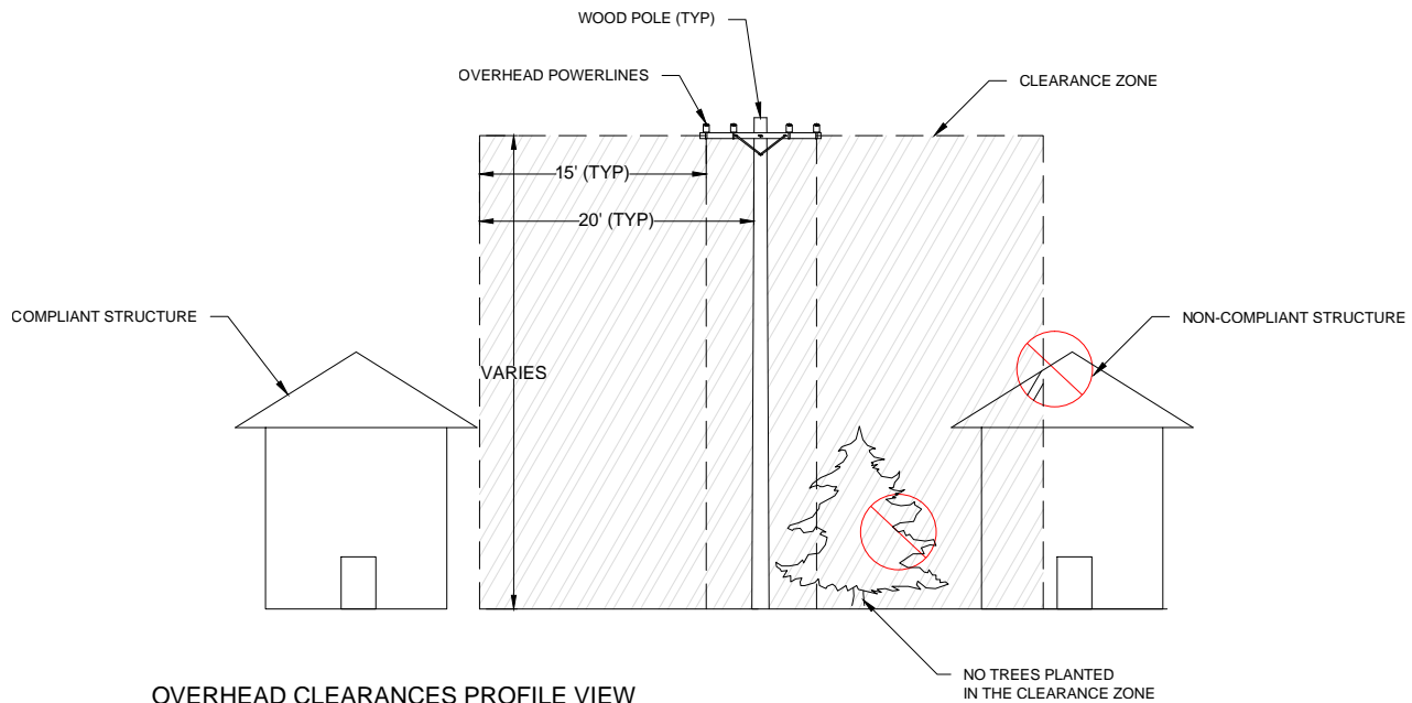
OVERHEAD CLEARANCES PROFILE VIEW
