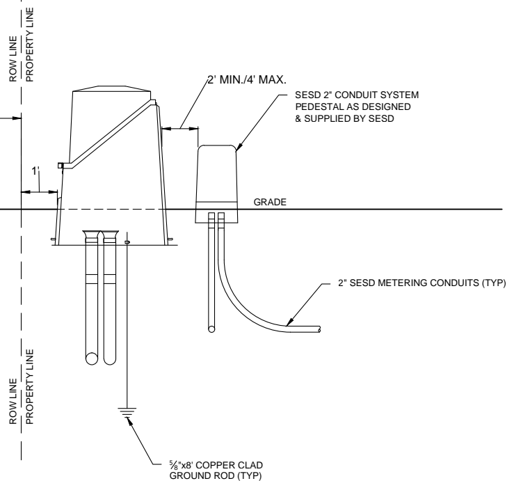
1 PHASE RIGHT ELEVATION VIEW
