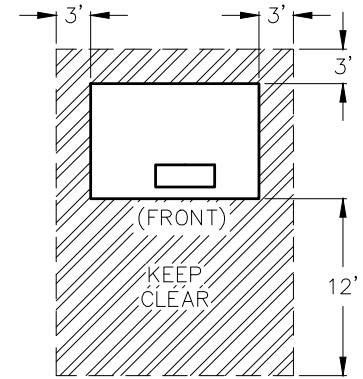
TYPICAL CLEARANCES
