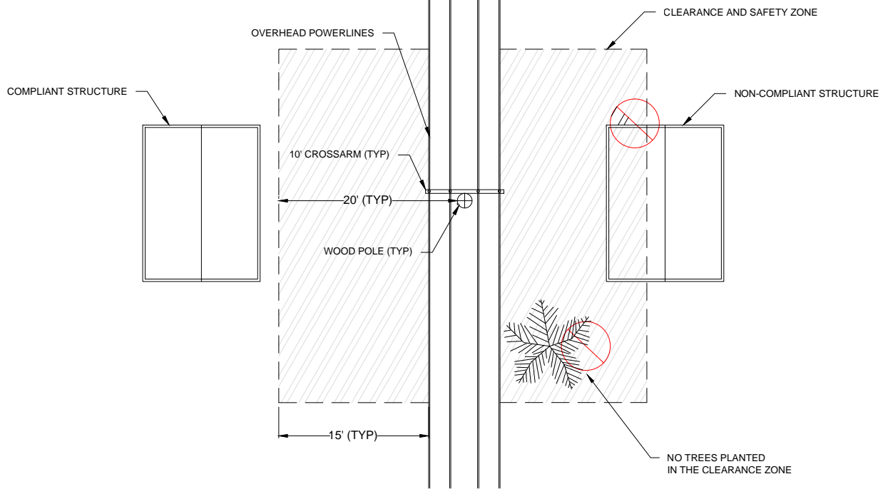
OVERHEAD CLEARANCES PLAN VIEW
