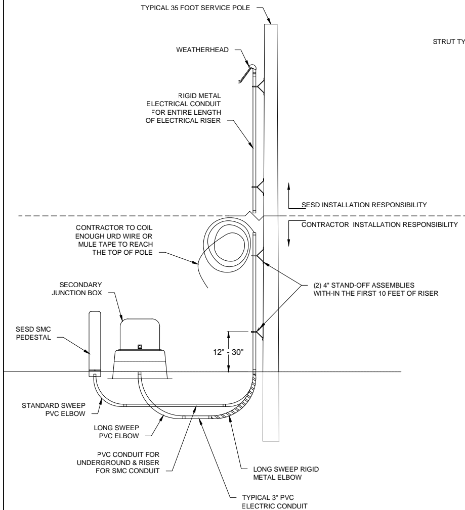
TYPICAL SERVICE POLE RISER
