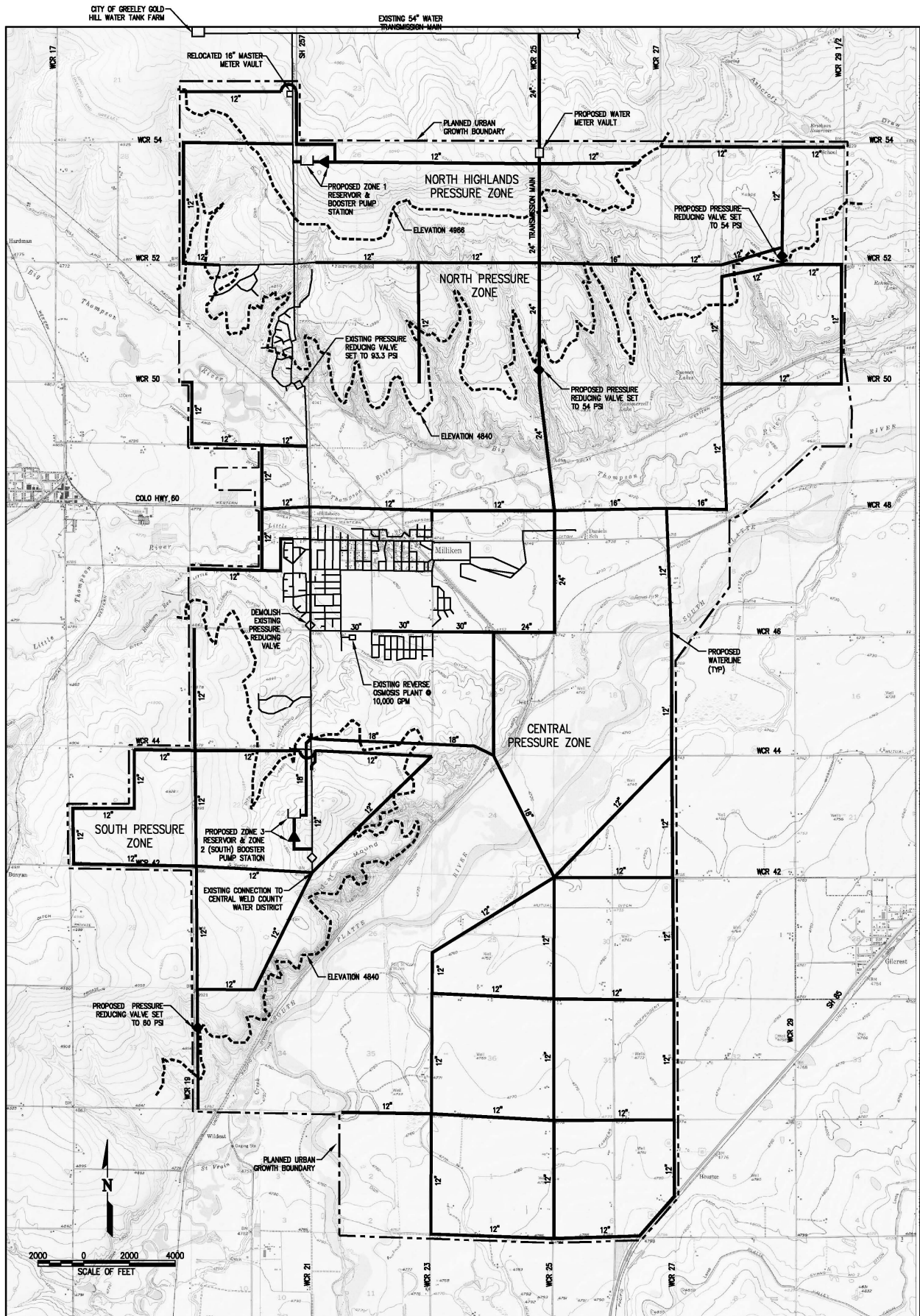
FIGURE 5-3 Town of Milliken Water & Sewer Master Plan Proposed Water System
