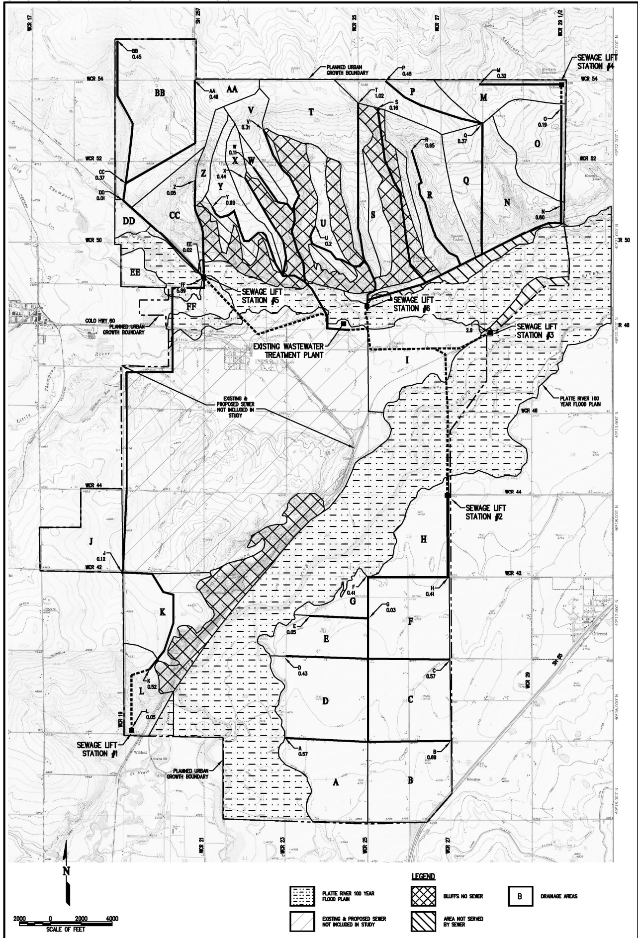
FIGURE 6-1 Town of Milliken Water & Sewer Master Plan Drainage Areas
